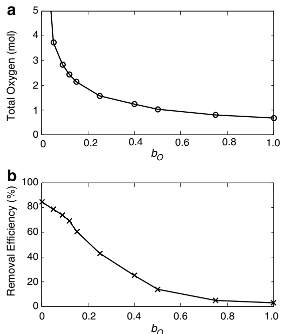
Fig. 11. Influence of the first-order oxygen decay constant ( b_0 ) on (a) the total moles of oxygen in the aquifer and (b) the removal efficiency of toluene in the subsurface prior to discharge.
